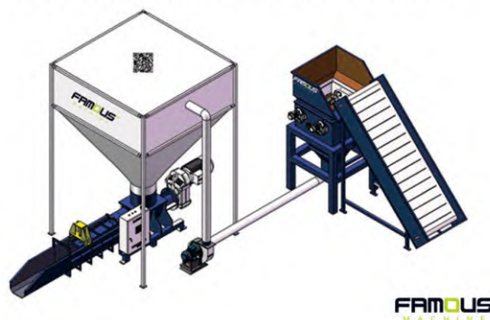
COMPACTOR WITH SILO SYSTEM
